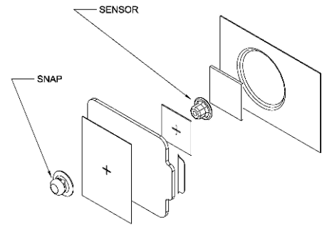
Figure 1: Schematic of Integrated ECG Electrode.
